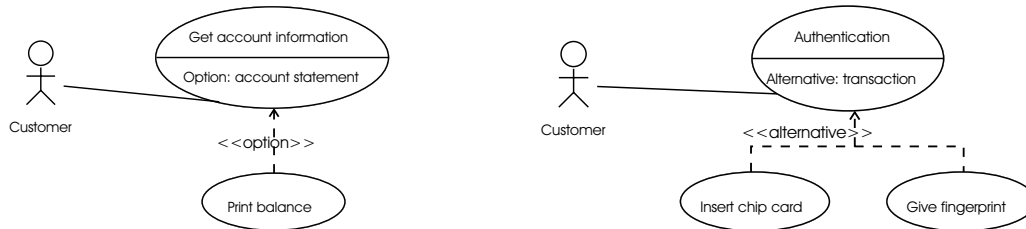
Modeling variability with extended UML Use Case diagrams
